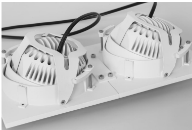
All directional tilt & air Dynamic heatsink;
